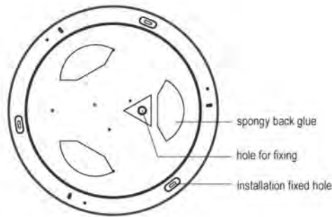
backside of the lamp body
